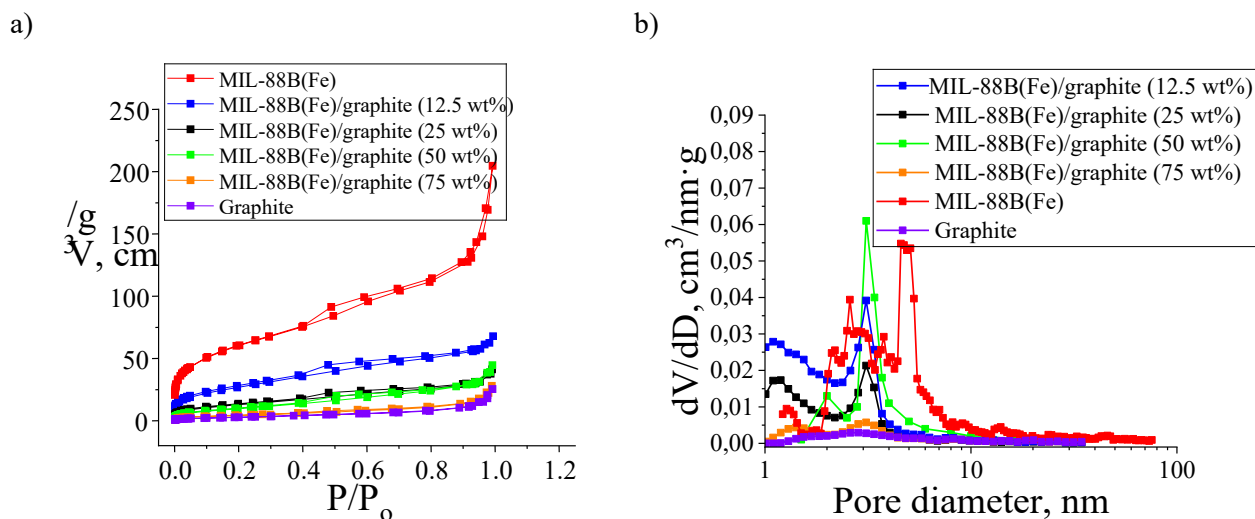
Figure 5. Nitrogen adsorption–desorption isotherms at 77 K (a) and differential pore size distribution curves for MIL-88B(Fe)/graphite composites (b)
