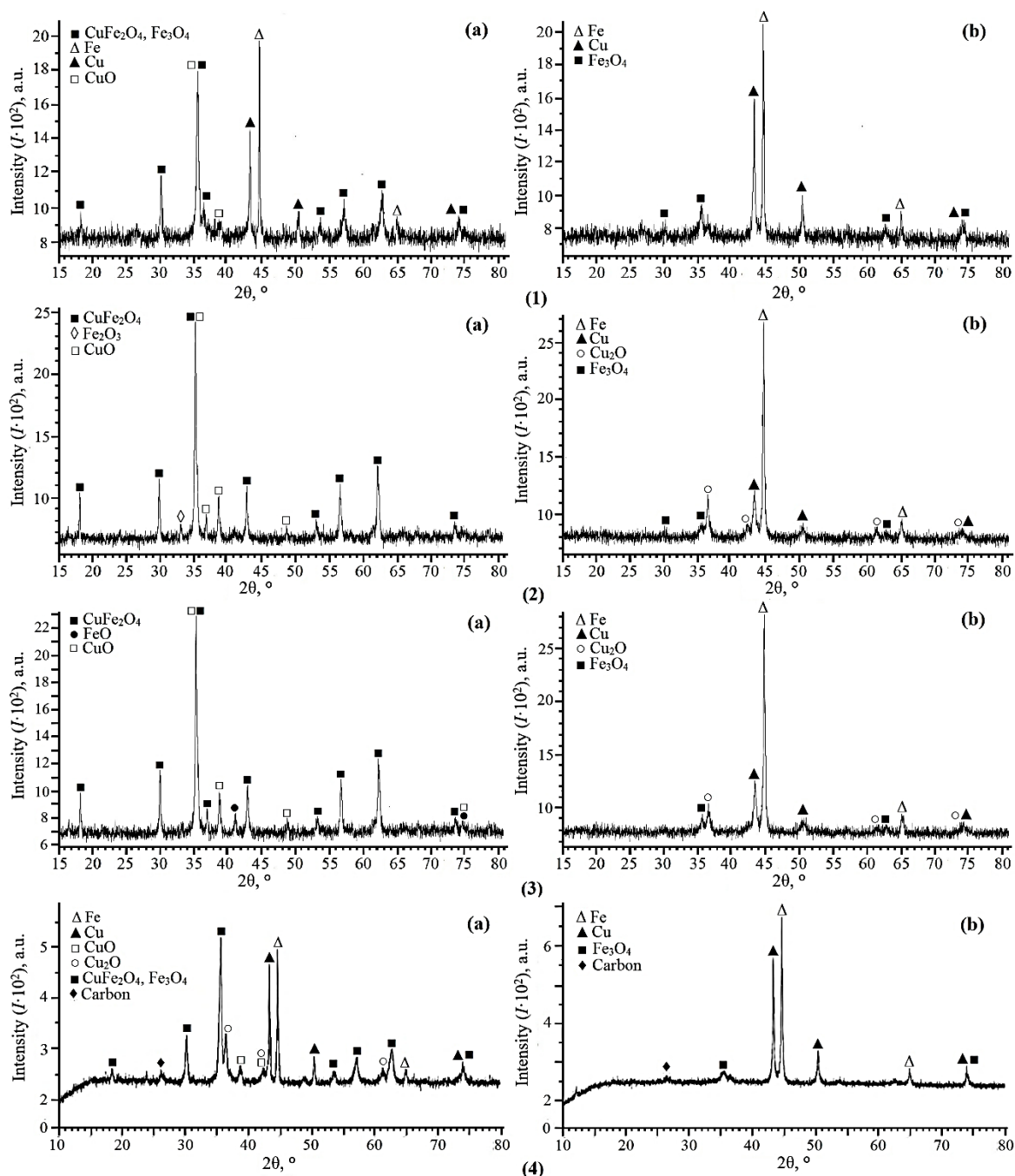
Figure 5. XRD patterns of \text{CuFe}_2\text{O}_4 + \text{PVA} (1), \text{CuFe}_2\text{O}_4 + \text{PVP} (2), \text{CuFe}_2\text{O}_4 + \text{PEG} (3), and \text{CuFe}_2\text{O}_4/\text{g-C}_3\text{N}_4 (4) after HT at 700 °C (a) and (b) after electrochemical experiments
