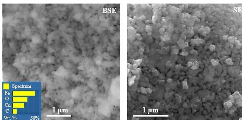
Figure 7. SEM images of \text{CuFe}_2\text{O}_4 + PVP (700 °C) sample
