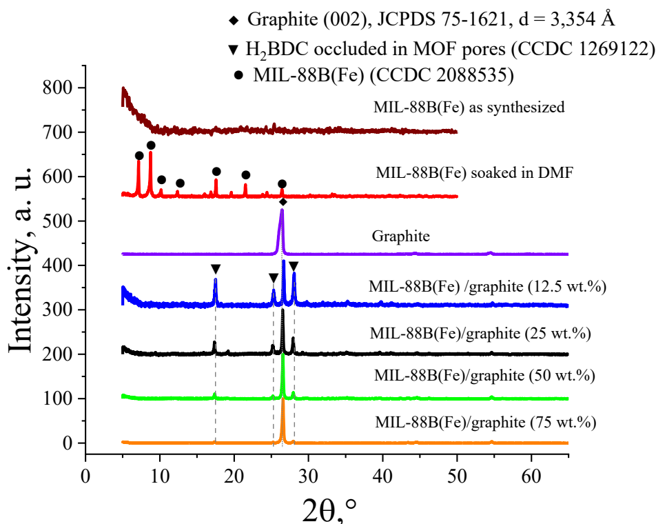
Figure 2. X-ray diffraction patterns of MIL-88B(Fe) and synthesized composites (CuK \alpha , \lambda = 1.5460 Å)
