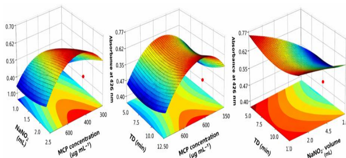
Figure 3. Response surface plots showing the effect of independent variables ( X_1 : MCP concentration, X_2 : \text{NaNO}_2 volume, X_3 : diazotization time) on the absorbance of the azo dye at 426 nm: (a) X_1 vs. X_2 at fixed X_3 ; (b) X_1 vs. X_3 at fixed X_2 ; (c) X_2 vs. X_3 at fixed X_1
