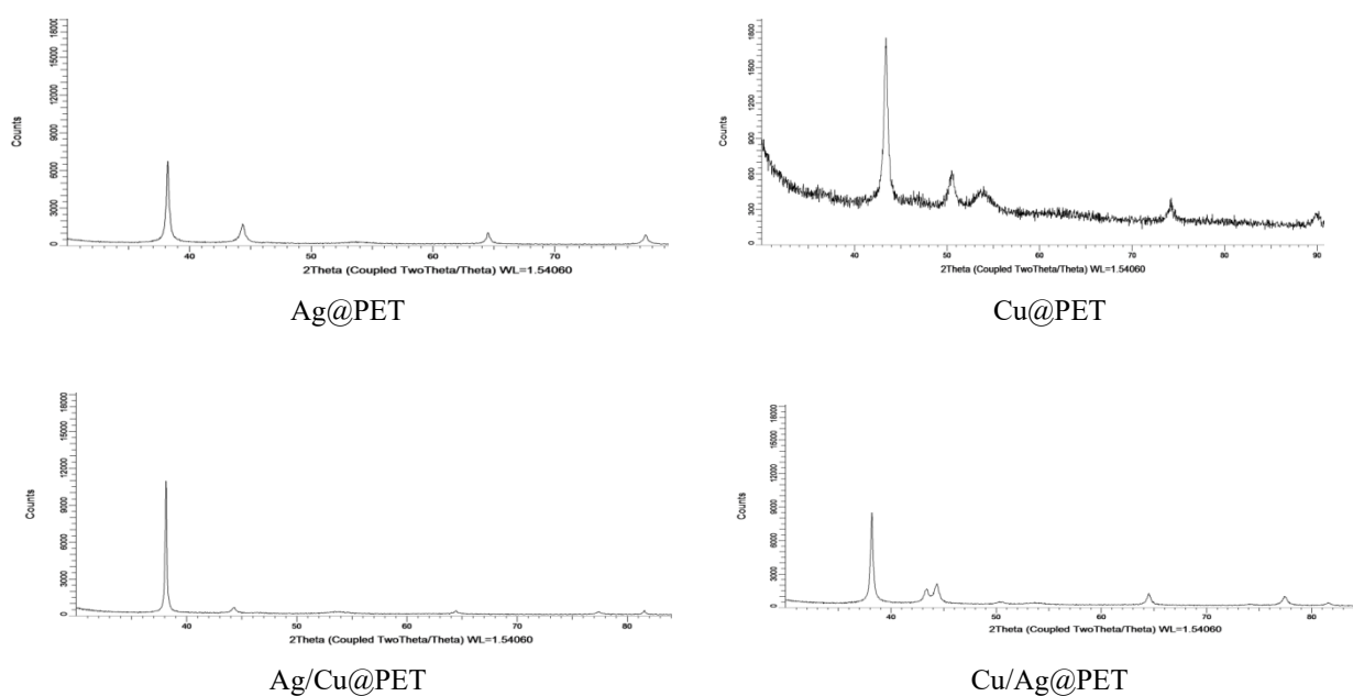
Figure S1. X-ray diffraction patterns of the studied composite membranes
